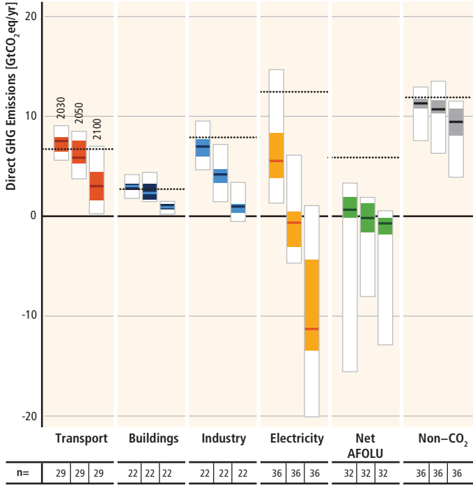
450 ppm CO 2 eq with CCS
